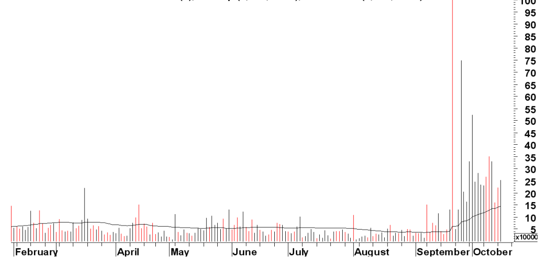
VOLUME DOWN (0), VOL Up (2,537,560.0), MA volume (1,449,277.4)
