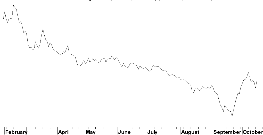
Relative Strength Comparative(VNINDEX) (0.015331, +0.000745)
